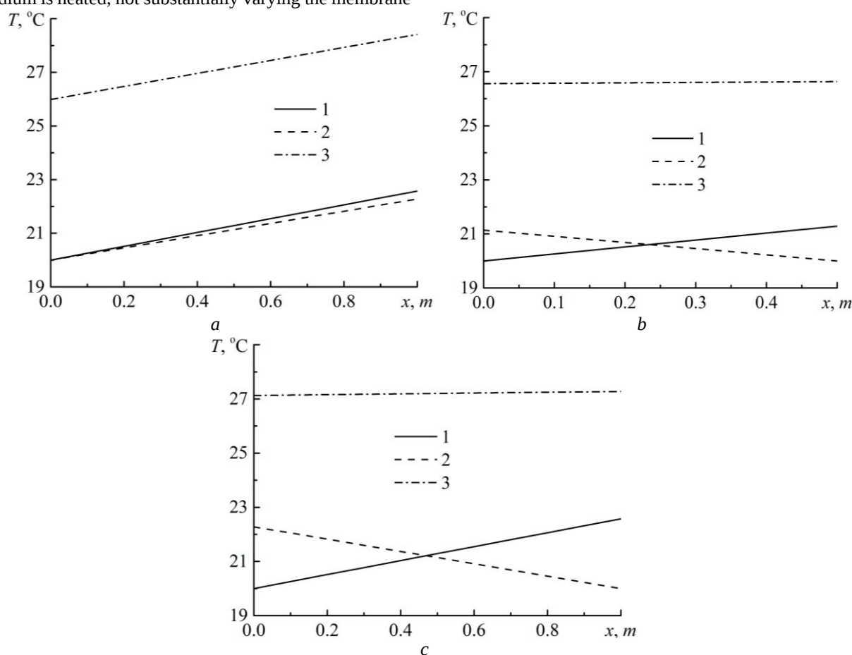
Figure 1. Temperature variation of the treated medium along the channels and the membrane (1 – temperature T_1 ; 2 – T_2 ; 3 – T_m ): a – co-current flow of the medium, b – co-current flow of the medium along the channel at L = 0.5 m, c – counter-current flow of the medium at L = 1 m.
